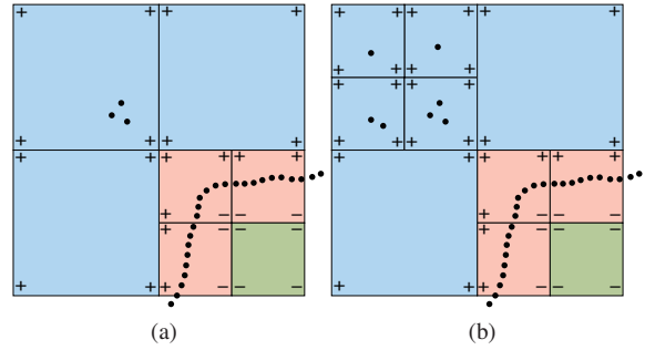
Figure 3: Outlier removal during the construction of the BOT. (a) An isolated outlier cell. (b) A cluster of the outlier cells.
