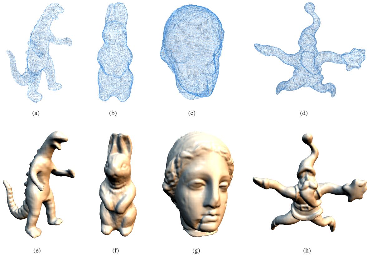
Figure 11: MPU implicit surfaces based on the BOTs shown through (e) to (h), which are reconstructed from the (a) DINOSAUR, (b) RABBIT, (c) IGEA and (d) SANTA data sets. The particles (shown in blue) used for visibility checks are rendered with the input data points (shown in gray).
