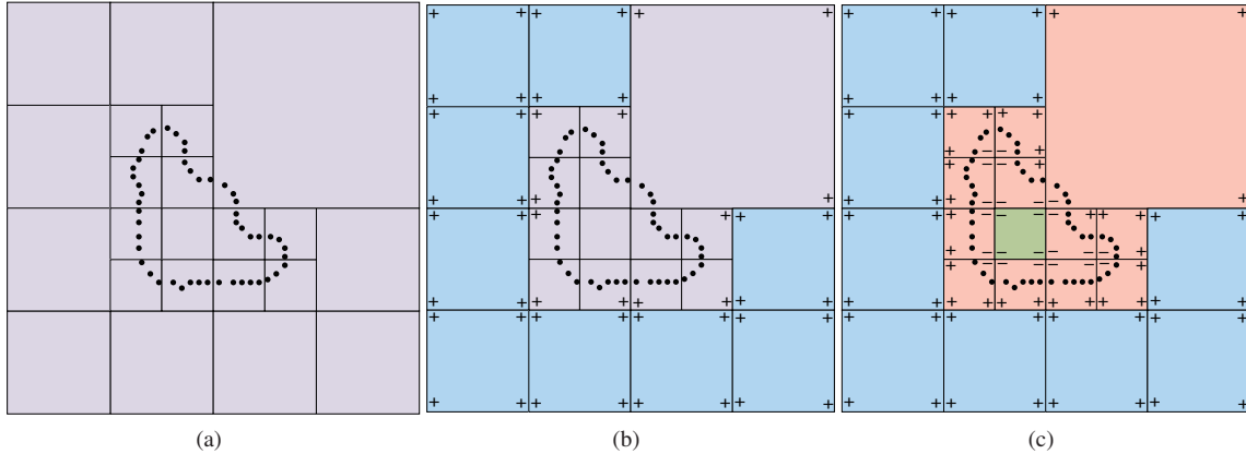
Figure 2: The construction process of a BOT. (a) Octree subdivision of a point set \mathcal{P} . (b) The growing process identifies a set of mono-oriented cells tagged as out (the blue cells with + tags). (c) The carving process resolves the remaining untagged corners and identifies the mono-oriented cells tagged as in (the green cell with - tags) and the bi-oriented cells (the red ones).
