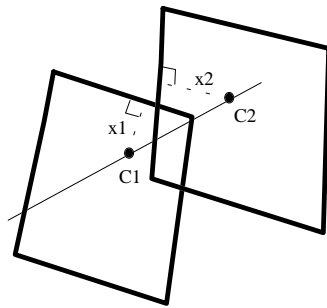
Fig. 6 result color = \frac{x_1^2 * C_1 + x_2^2 * C_2}{x_1^2 + x_2^2} , (where x_1, x_2 are distances from the hit pixels to their nearest borders.)
